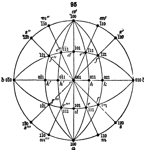
Stereographic Projection of Faces on Chrysolite Crystal, Fig. 94
